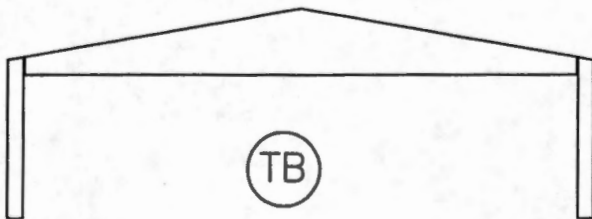
TAPERED BEAM FRAME, CONSTANT DEPTH COLUMN AND RAFTER WITH HORIZONTAL BOTTOM CORD MAXIMUM WIDTH 60'
