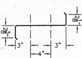
10" ZEE OR CEE
