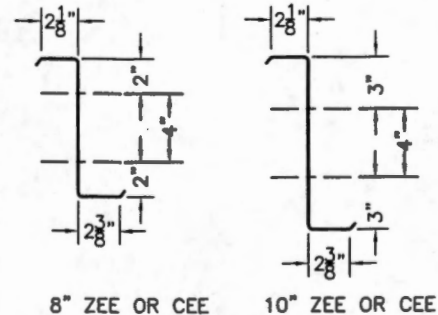
8" ZEE OR CEE 10" ZEE OR CEE
