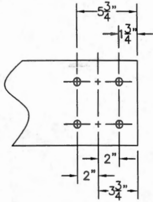
#4 PUNCH QUAD PUNCH
