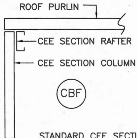
LEAN-TO FRAME WITH SHEAR CONNECTION AT TOP OF COLUMN
