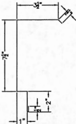
8" CANOPY RAKE FOR R PANEL
