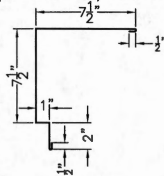
HIGH SIDE EAVE TRIM (8" CHANNEL) R PANEL
