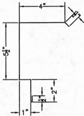
8" CANOPY RAKE FOR R PANEL
