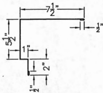
HIGHSIDE EAVE TRIM (6" CHANNEL) R PANEL
