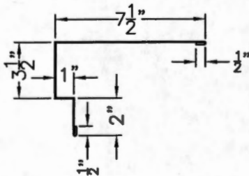
HIGHSIDE EAVE TRIM (6" CHANNEL) R PANEL
