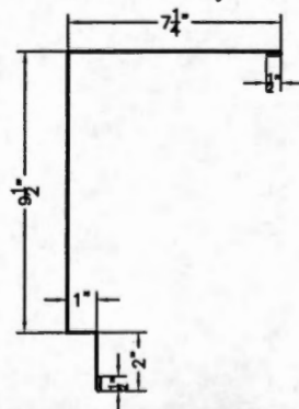
HIGH SIDE EAVE TRIM (10" CHANNEL) R PANEL
