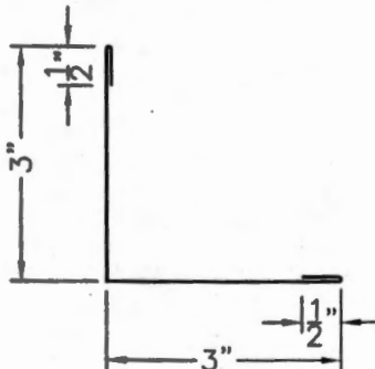
3" X 3" OUTSIDE L TRIM
