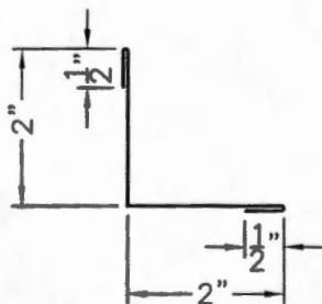
2" X 2" INSIDE L TRIM
