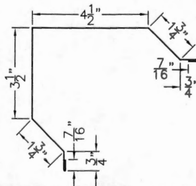
R PANEL CORNER TRIM
