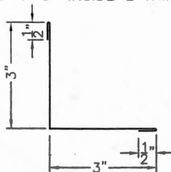
3" X 3" INSIDE L TRIM
